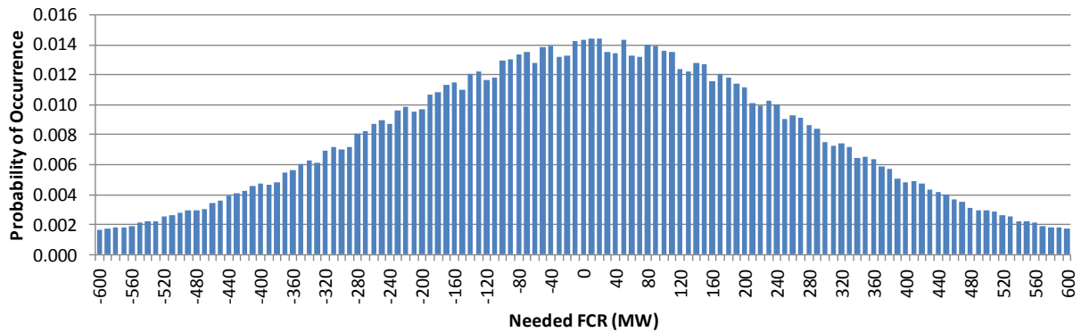
Figure 14: Probability distribution of the needed FCR due to market induced unbalances from -600 to 600 MW.
