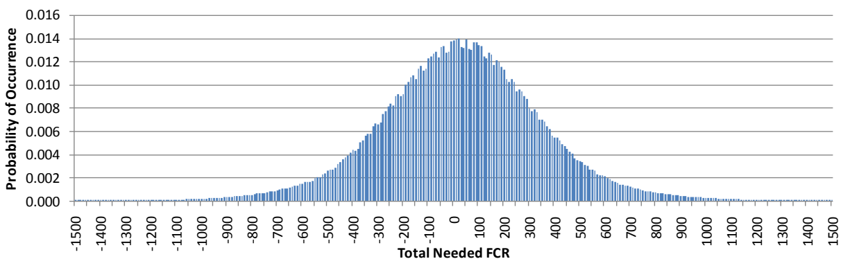
Figure 15: Probability distribution of the total FCR from -1500 to 1500 MW in RG CE.
