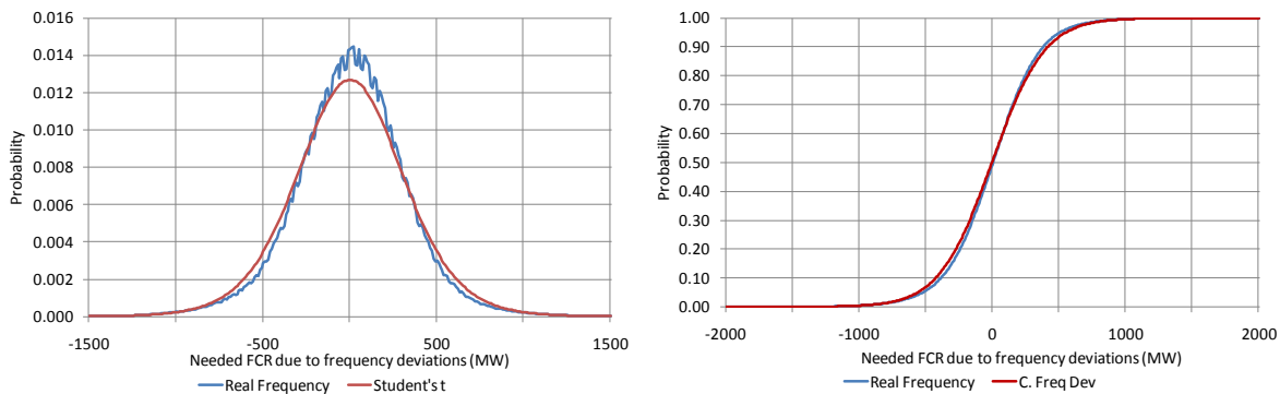
Figure 16: Probability distribution and cumulative distribution of the FCR needed due to the real frequency deviations in 2010 not associated with sudden generation trips and the Student's t distribution to which these values were adjusted.
