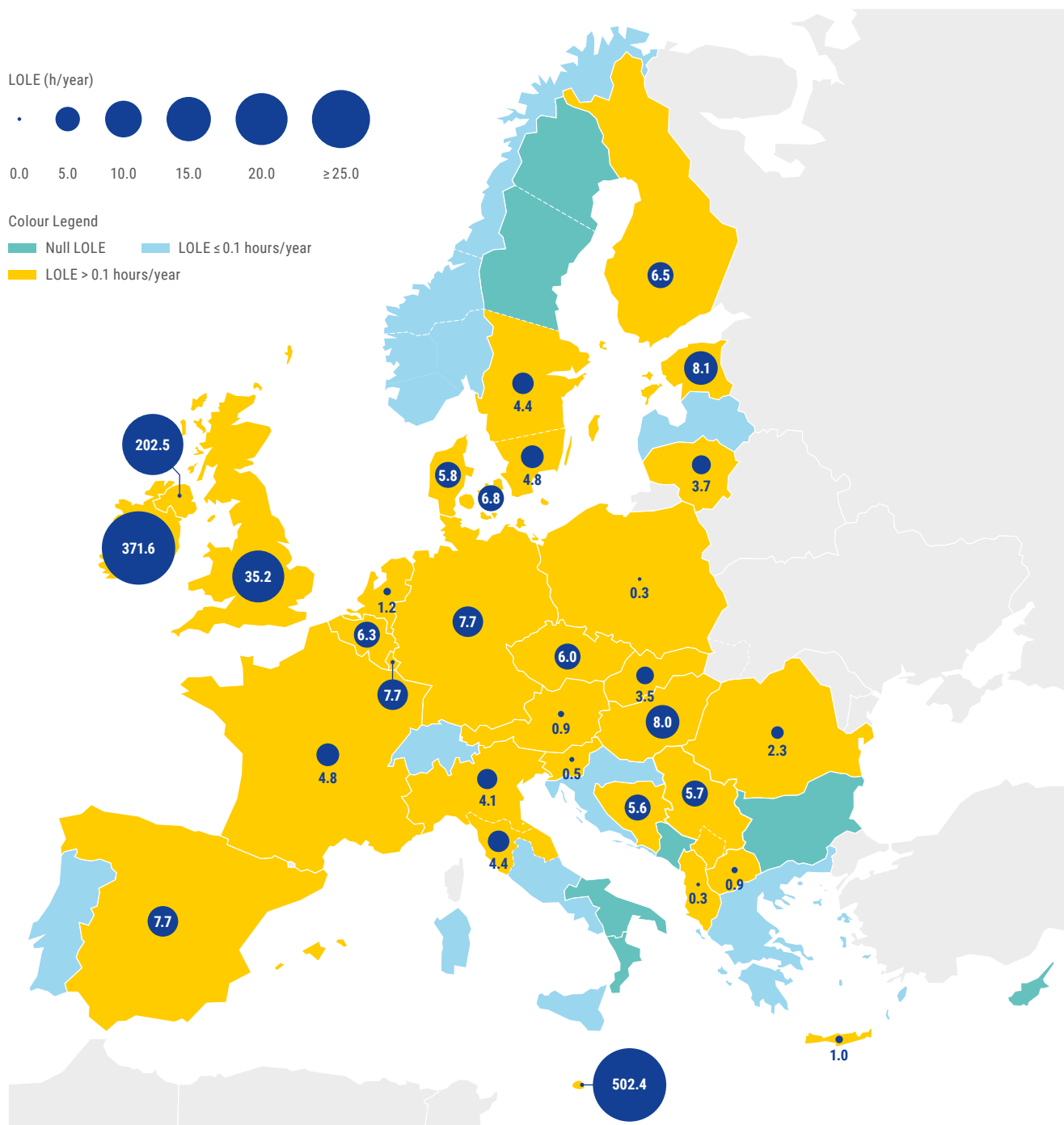
Figure 7: LOLE values in 2025* (Scenario B – Sensitivity)
