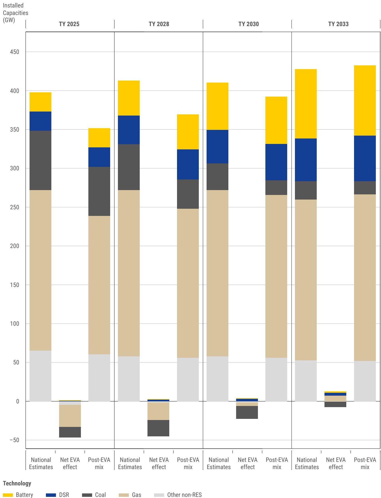
Figure 1: Net effect of the EVA on the European Perimeter – focus on technologies assessed (Scenario A – Central Reference)
