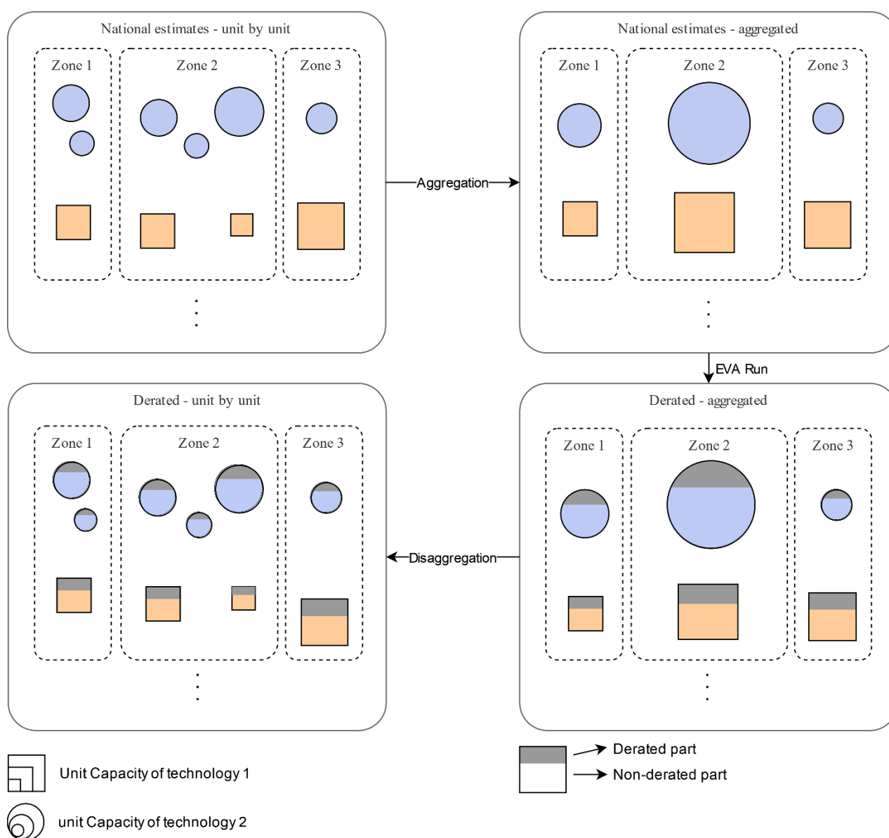
Figure 18: EVA unit aggregation process
