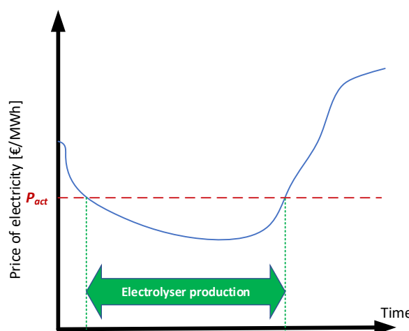
Figure 13: Activation price approach
