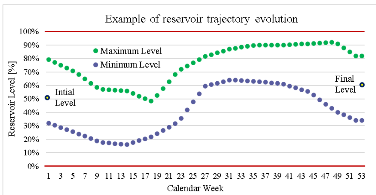
Figure 11: Example of reservoir trajectories and constraints
