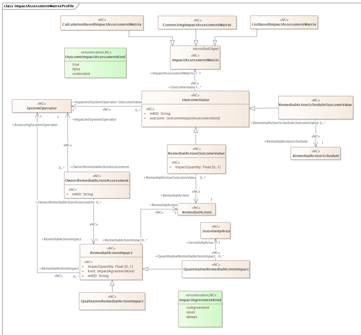
Figure 1 – Class diagram ImpactAssessmentMatrixProfile::ImpactAssessmentMatrixProfile
